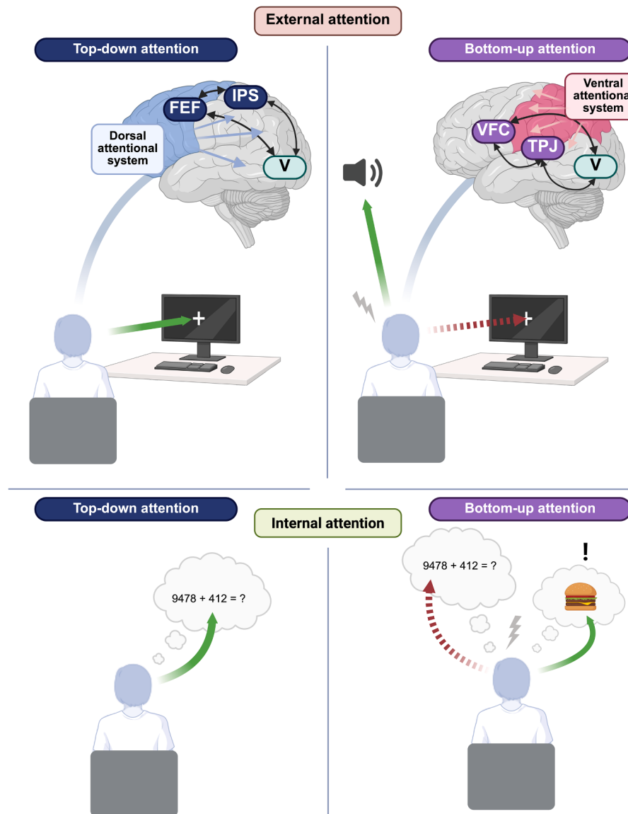
Fig. 1. A schematic overview of attentional functions, targets, and neural correlates. The top-left panel illustrates top-down external attention, where attention is voluntarily directed toward a perceptual target (e.g., a fixation cross), supported by the dorsal attentional system, which includes the frontal eye fields, intraparietal sulcus, and visual system. The top-right panel depicts an example of bottom-up external attention, in which a sudden external stimulus (e.g., sound) captures attention involuntarily, mediated by the ventral attentional system, involving the ventrolateral prefrontal cortex, temporoparietal junction, and visual system. The bottom-left quadrant represents top-down internal attention, where goal-directed focus is allocated to internally generated content (e.g., mental arithmetic). The bottom-right quadrant illustrates bottom-up internal attention, where attention is involuntarily diverted by internally generated thoughts (e.g., a hunger signal). FEF = frontal eye fields; IPS = intraparietal sulcus; TPJ = temporoparietal junction; V = visual cortex; VFC = ventral frontal cortex.
